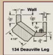
Detail of No. 134 Deauville Leg
