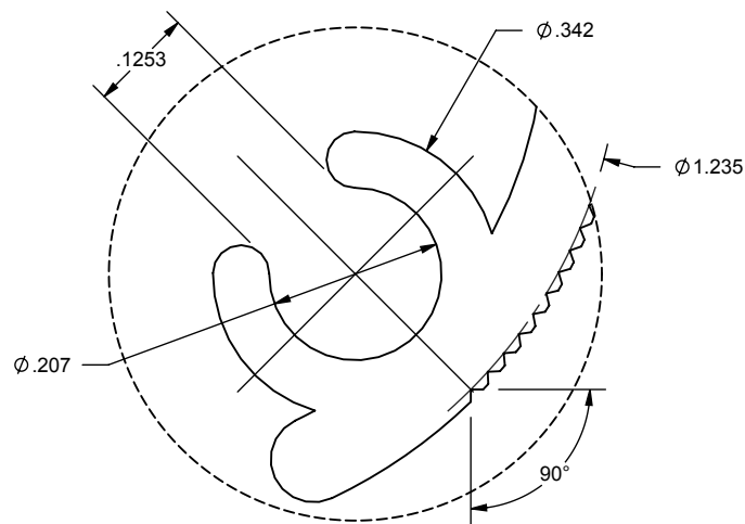
DETAIL A SCALE 4 : 1 TYP.
