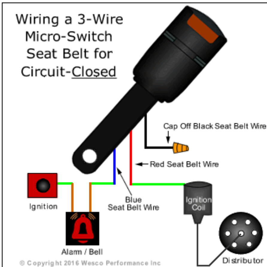
Below Circuit- Closed Diagram
