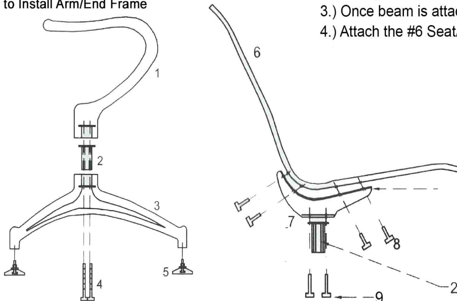
How to Install Arm/End Frame
