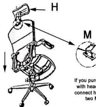
6.) Connect the seat/back upper portion and base/gas cylinder lower portion together by lining up with hole in mechanism. Set upper portion over lower portion and push down. Carefully sit in the chair to pressure fit together.
