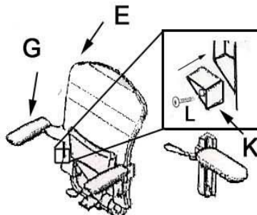
4. Slide armrests onto notched sides of backrest & screw in both K - Armrest Stoppers using one L screw each.
