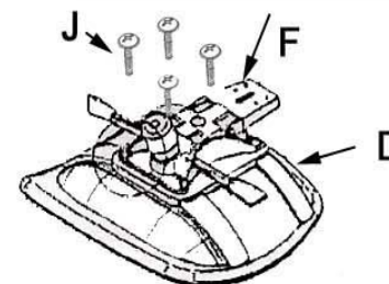
3.) Attach mechanism to seat cushion using four J bolts.
