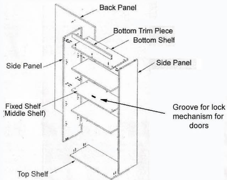
Exploded diagram of parts: (doors not shown)
