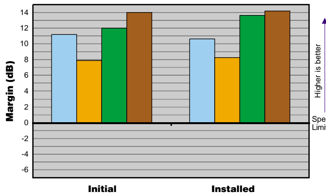
Belden DataTwist 350 Cat 5e Return Loss Margin (20-100MHz)
