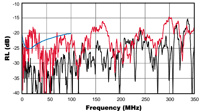
Industry Cat 5e Cable Return Loss
