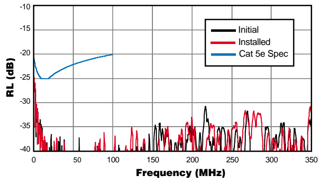
Belden DataTwist® 350 Return Loss
