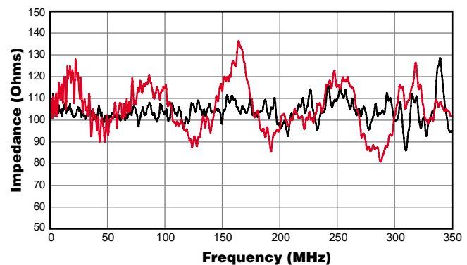
Industry Cat 5e Cable Impedance
