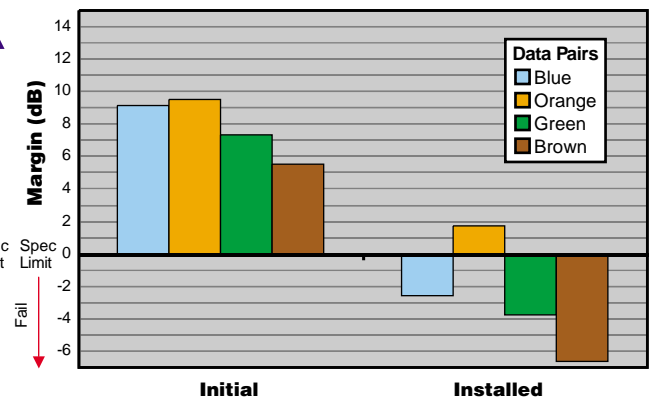
Industry Cat 5e Cable Return Loss Margin (20-100MHz)
