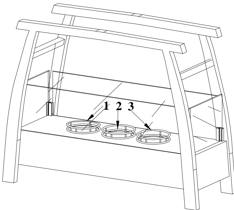
Figure 3 –Fuel Canister Installed
