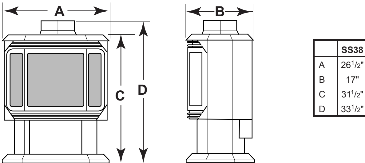
Figure 2 - External Stove Dimensions
