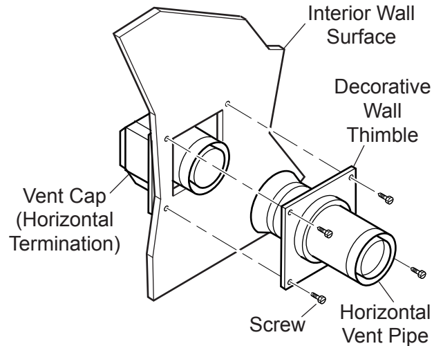
Figure 14 - Connecting Vent Cap with Horizontal Vent Pipe
