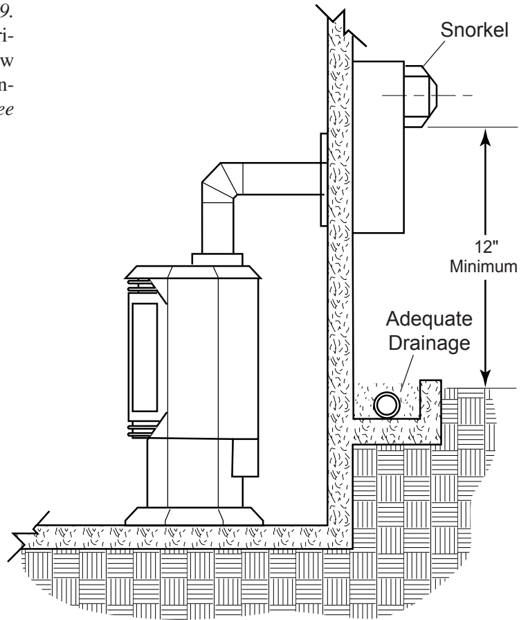
Figure 9 - Snorkel Termination with Drainage Pipe
