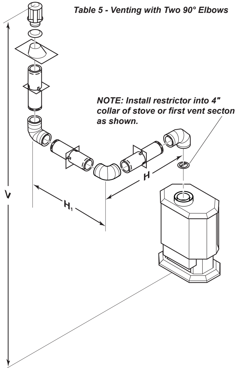
Figure 24 - Vertical Rigid Venting Configuration Using Three 90° Elbows with Two Horizontal Runs
