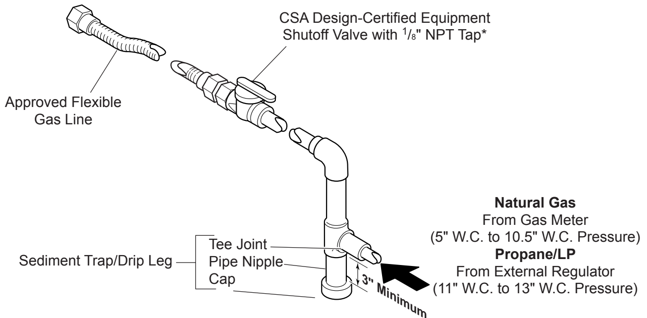
Figure 28 - Gas Connection
