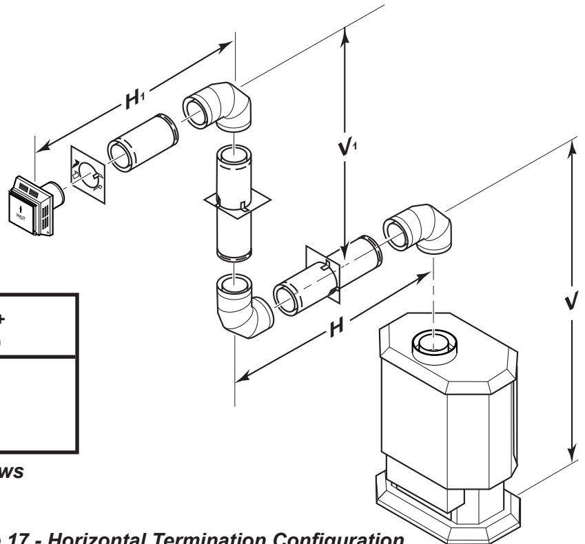
Figure 17 - Horizontal Termination Configuration for Rigid Venting Using Three 90° Elbows with Termination at 90° with Stove
