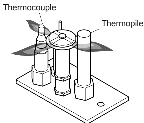
Figure 46 - Typical Pilot Flame
