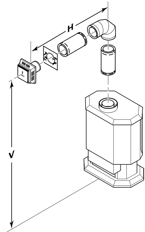
Figure 15 - Horizontal Termination Configuration for Rigid Venting Using One 90° Elbow
