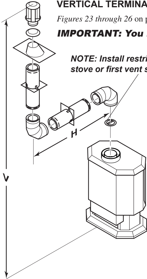
Figure 23 - Vertical Rigid Venting Configuration Using Two 90° Elbows
