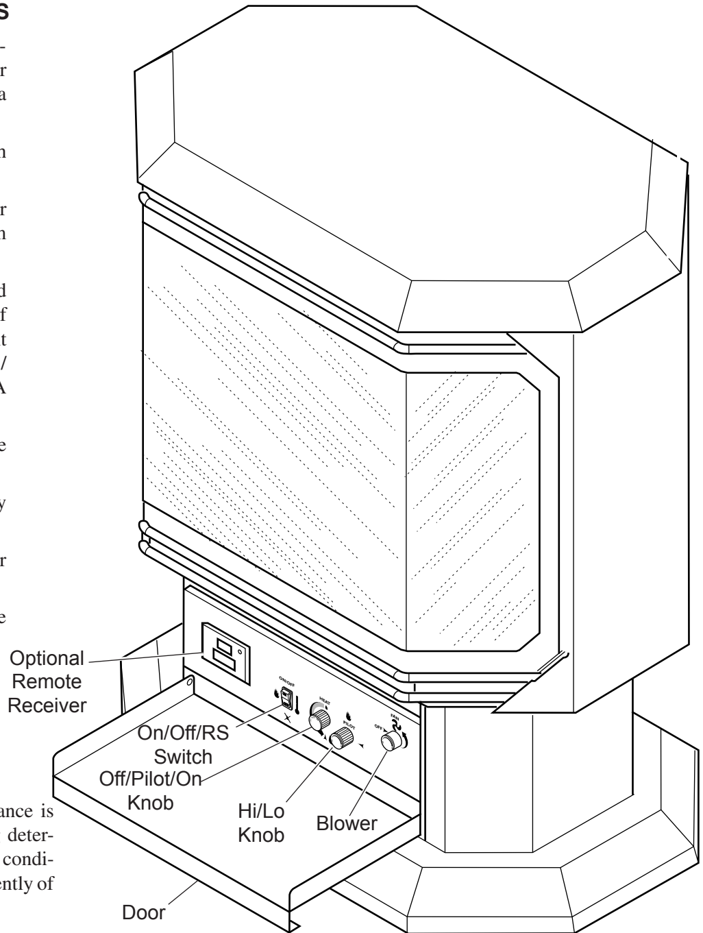
Figure 1 - SS38 Stove
