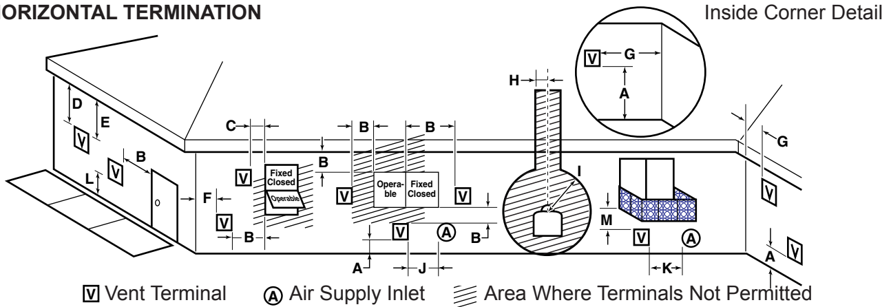
Figure 6 - Horizontal Vent Termination Location
