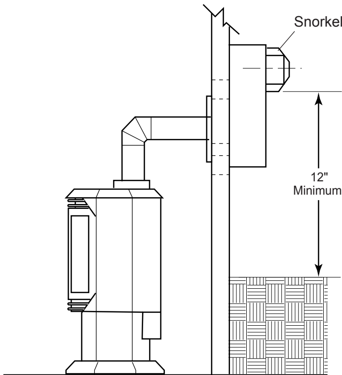
Figure 8 - Snorkel Termination
