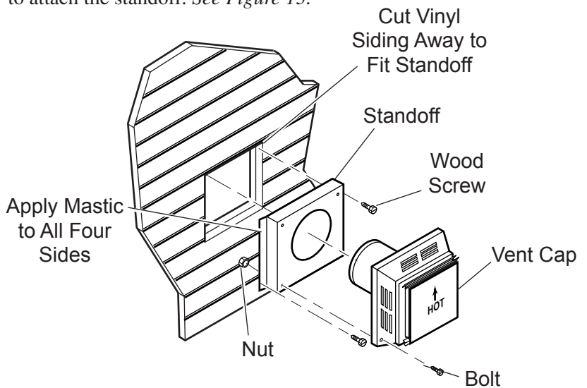
Figure 13 - Installing Vinyl Siding Standoff
