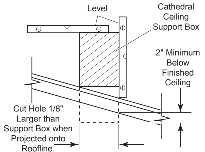
Figure 21 - Cathedral Ceiling Support Box Installation
