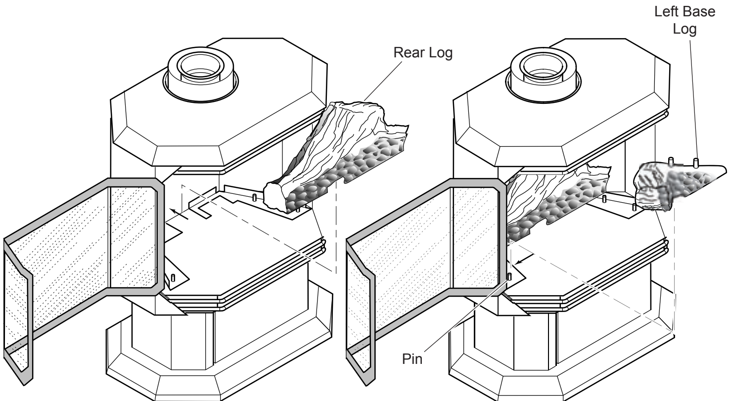
Figure 32 - Installing Rear Log
