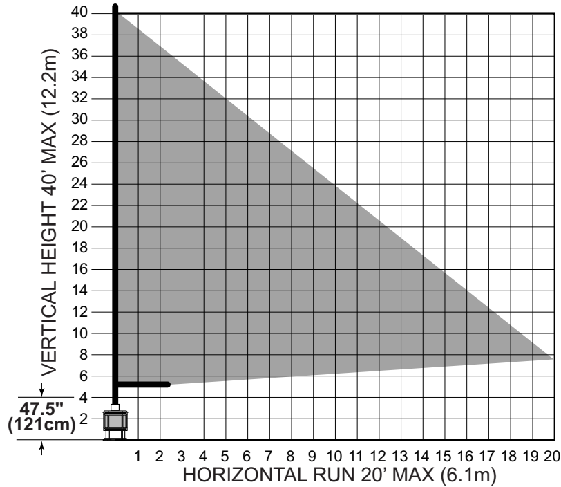
Figure 7 - Allowable Venting Chart
