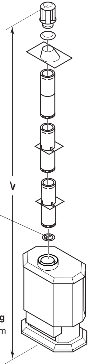
Figure 26 - Vertical Rigid Venting Configuration with No Horizontal run
