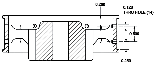
Section L-L
