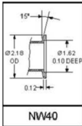
PORT SIZE FOR ASM182TD+
