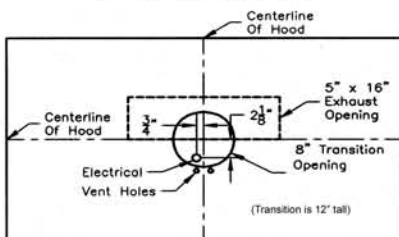
T200 Dual Blower Top View Straight Line, Professional
