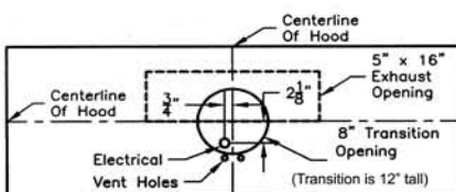
T200 Dual Blower Top View Slope Line, Flair Line, Convex, Emerald, and Excalibur
