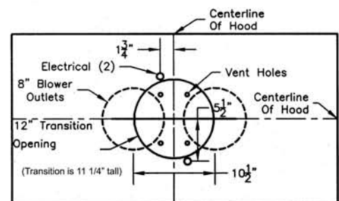
T400 Cluster Blower Top View
