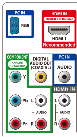
Rear Panel
