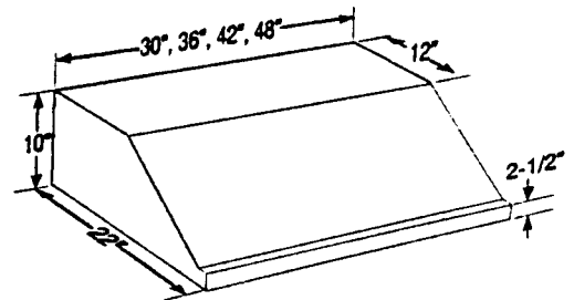
K210A series hood
