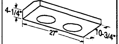
Model P8 blower / rough-in kit
