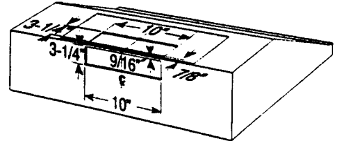
K210A series hood
