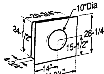
Models EB6 & EB9 exterior blowers
