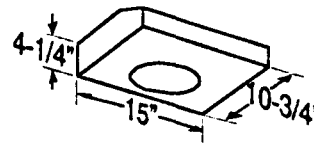
Model P5 blower / rough-in kit
