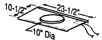
Exterior blower rough-in kit
