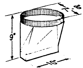
Model 412/413 3-1/4" x 10" to 7"8" Rd. transition
