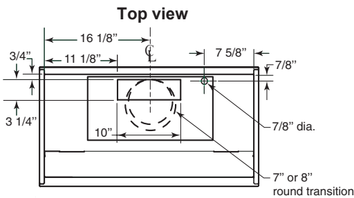
MODEL PIK33 WITH P5 BLOWER (Vertical Outlet)
