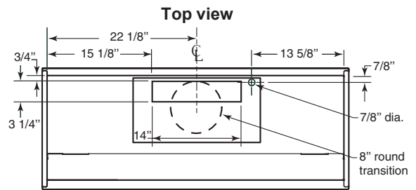
MODEL PIK45 WITH P8 BLOWER (Vertical Outlet)
