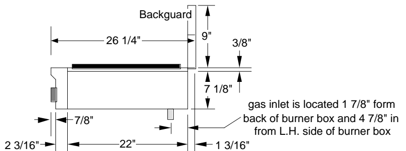
Front and Side View of Cooktop and Backguard (not to scale)
