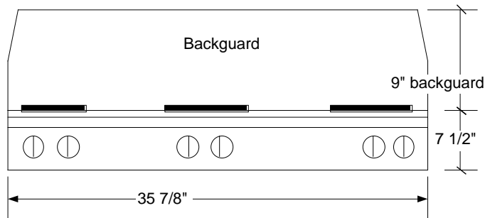
Front and Side View of Cooktop and Backguard (not to scale)
