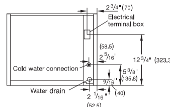
ED 220 as seen from behind:
