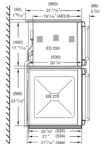
ED 220 as seen from the side:
