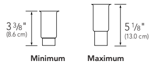
Adjustable legs
