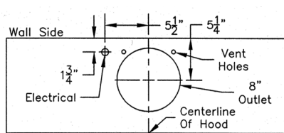
600 CFM B200 Dual Blower (Top View)
