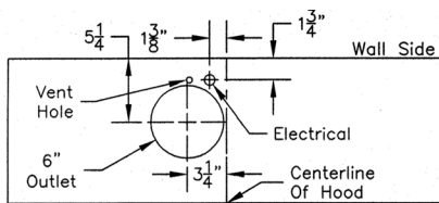
300 CFM B100 Single Blower (Top View)
