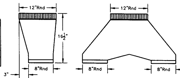
VP563 Transition (Optional) For B400 (B200 Dual Blower & B200 Dual Blower)
