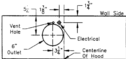
Top View--B100 Single Blower
