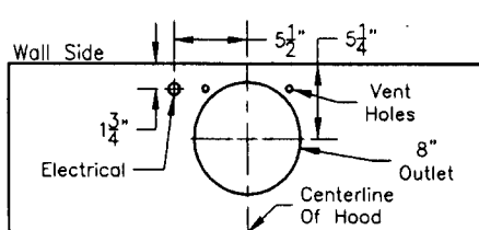
Top View--B200 Dual Blower
