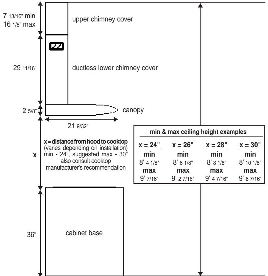
FIGURE 5 DUCTLESS INSTALLATIONS
