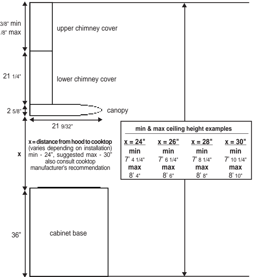
FIGURE 4 DUCTED INSTALLATIONS
