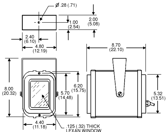
EH4007 DIMENSION DRAWING
