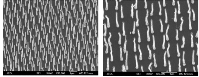
Fig. 4. SEM images of low (left) and medium (right) magnifications of carbon nanotube arrays.
