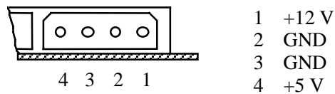
Figure 2 - Power Connector
