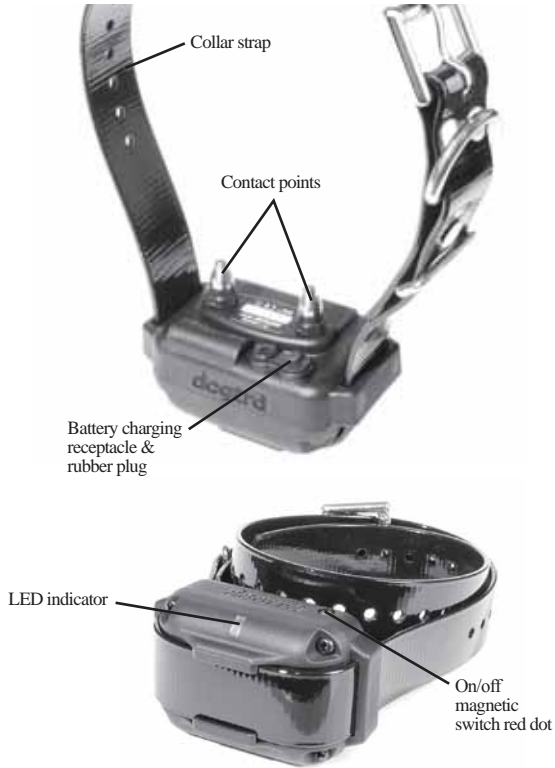
Receiver/Collar
