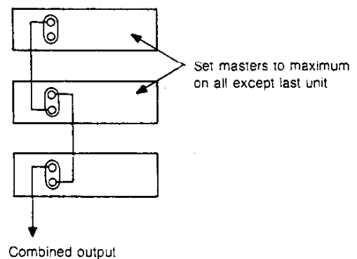
Figure 5 — Series-connected outputs
