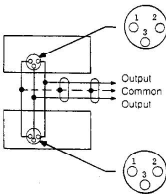
Figure 8 — Paralleled microphone outputs
