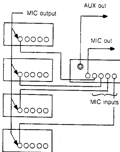
Figure 7 — Cascade-connected outputs
