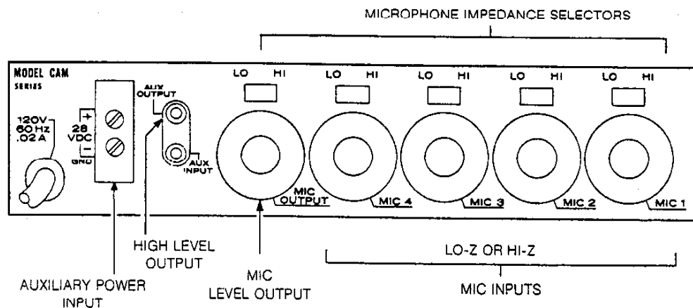
Figure 2 — CAM, rear chassis
