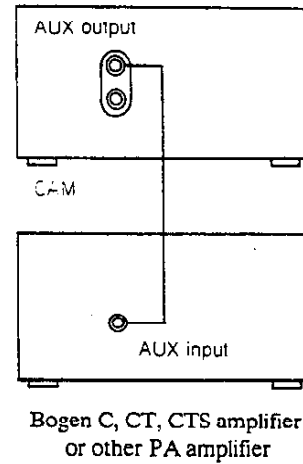
Figure 4 — Single connection for increased inputs
