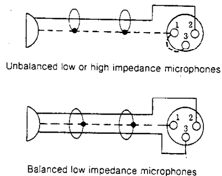
Figure 1 — Connecting microphone cables
