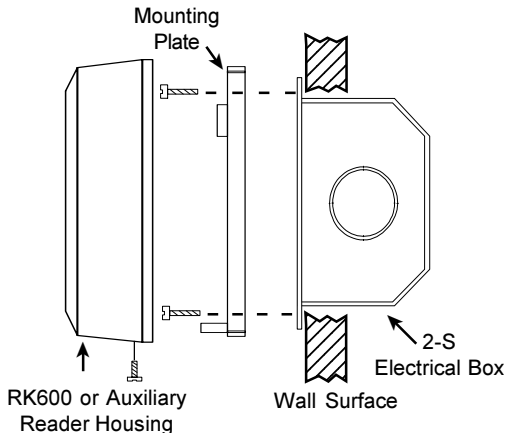
Figure 4 - Basic Installation
